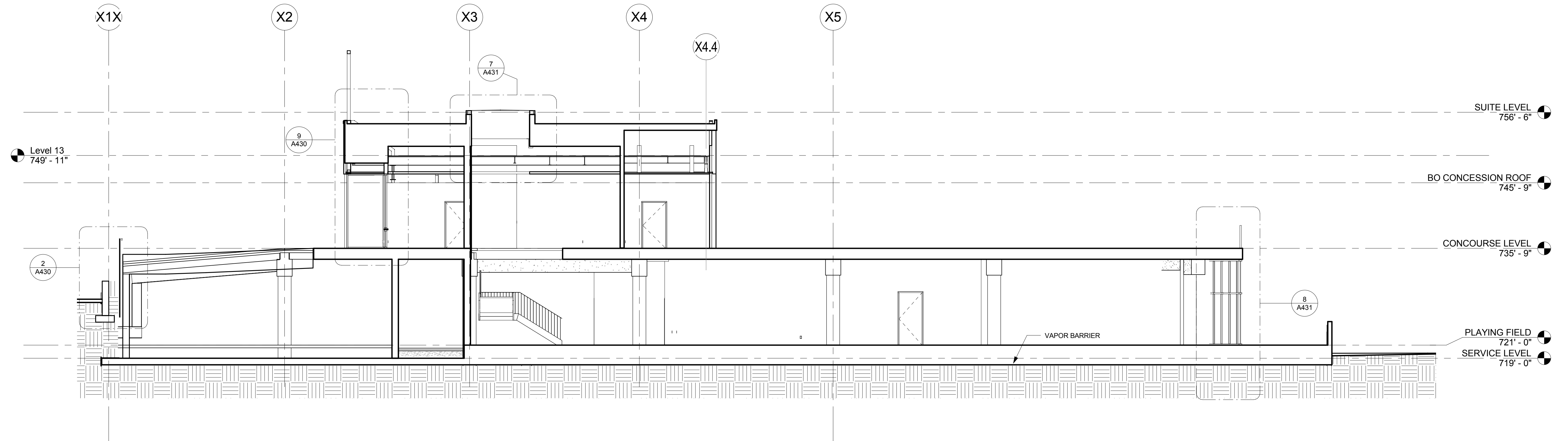
1 SECTION AT OFFICE W-E A410 1/8" = 1'-0"
