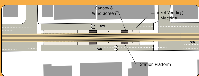
FIGURE 2.1 - Illustrative Raymond Center Platform Configuration
