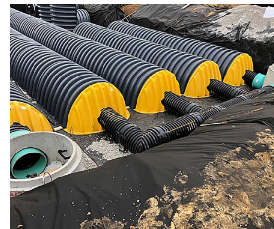
B : UNDERGROUND STORAGE Highly impervious light industrial and residential sites may use underground storage methods to effectively manage the sites' stormwater loads.
