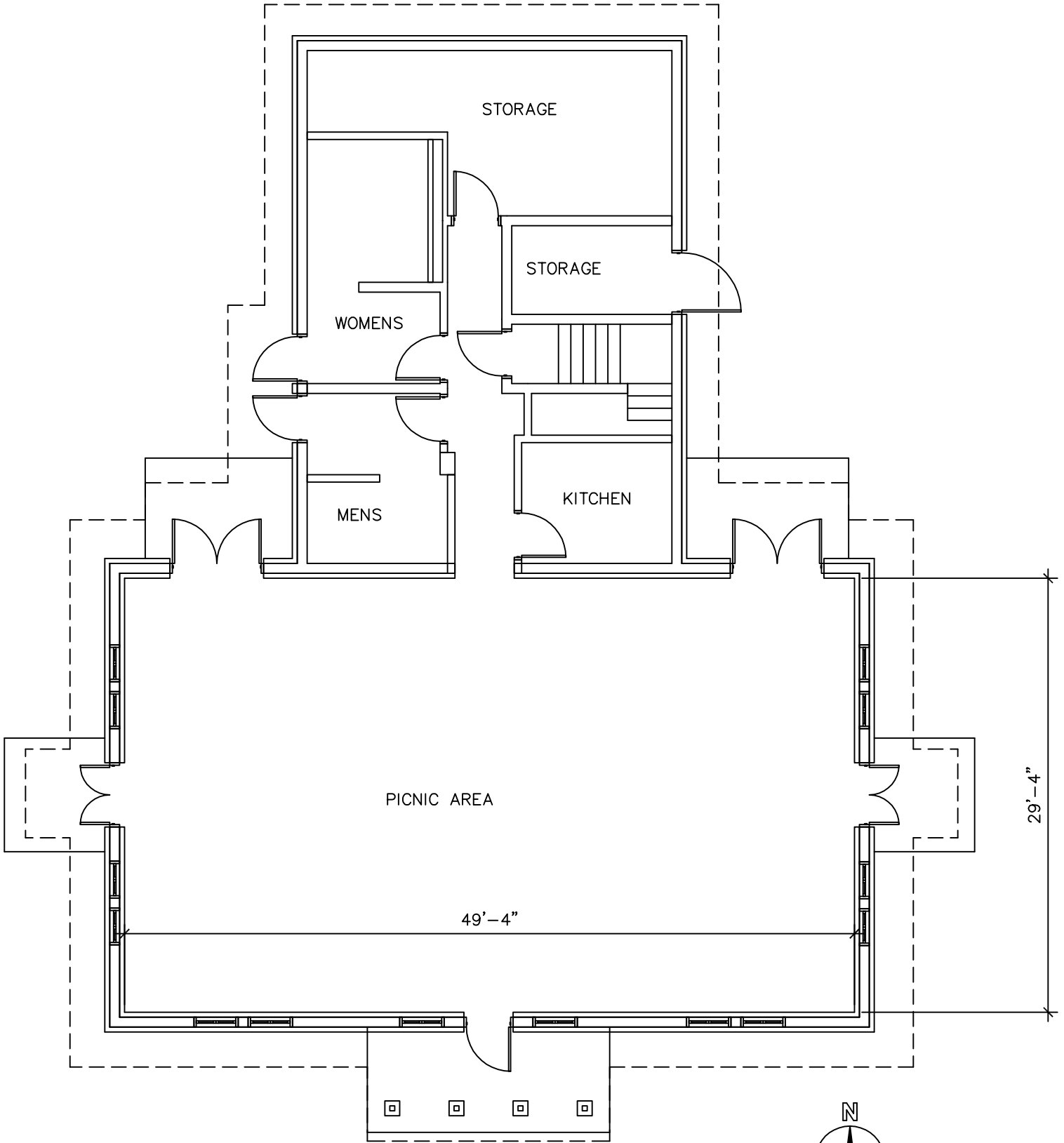
1 NEWELL PARK REC CENTER - FLOOR PLAN NO SCALE
