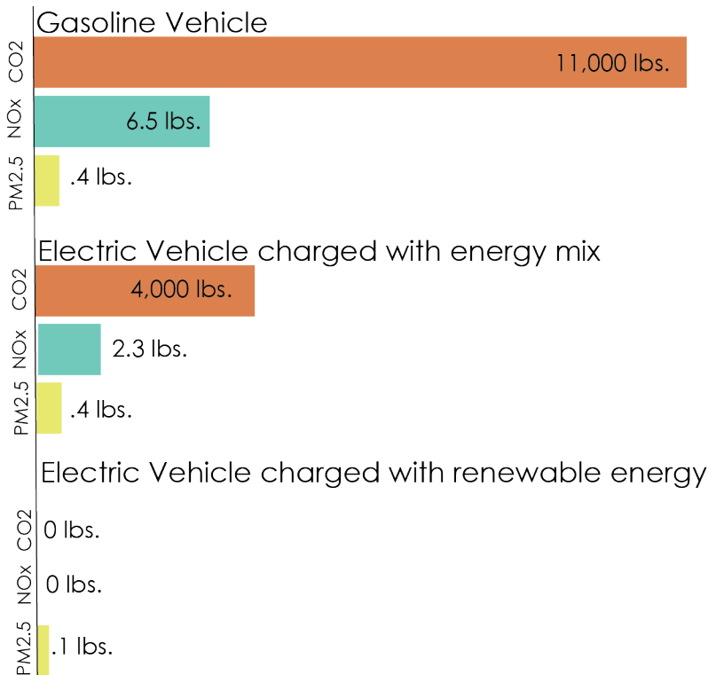
Annual emissions by fuel type (12,000 miles for compact/midsize car)
