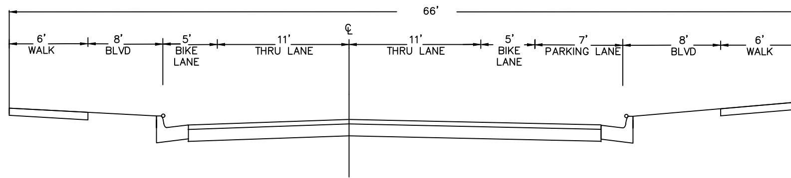
EXISTING CROSS SECTION
