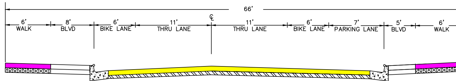
PROPOSED CROSS SECTION
