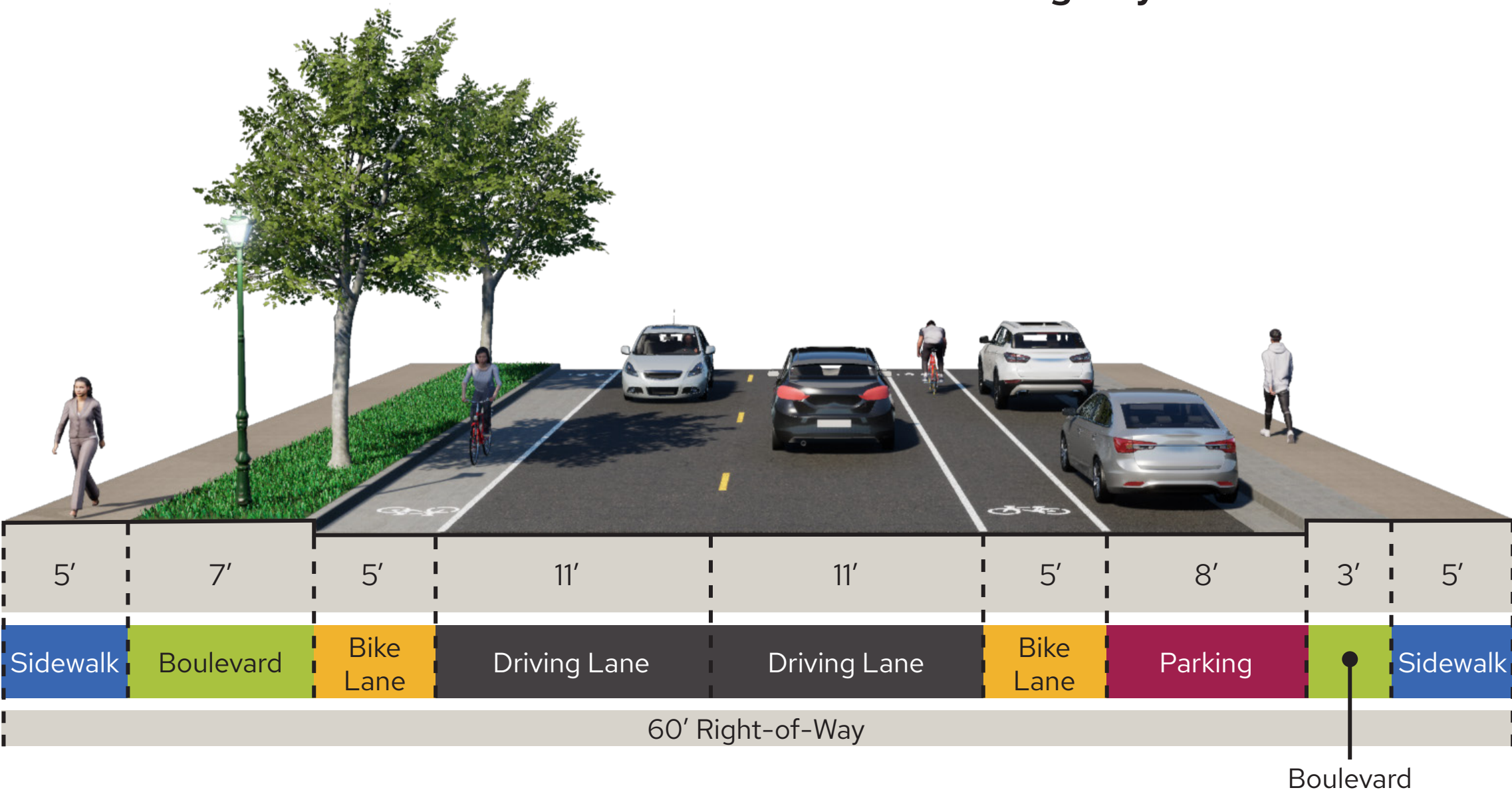
On-Street Bike Lanes with a Parking Bay
