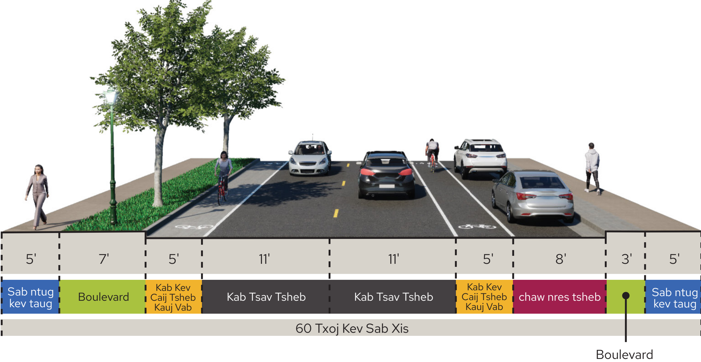
Ntawm-Street Bike Cov Kab Kev nrog Parking Bay
