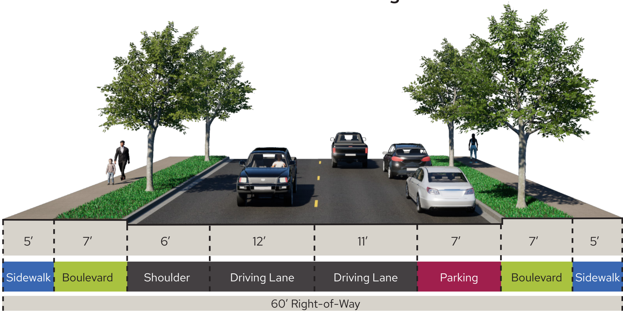
Current Street Design
