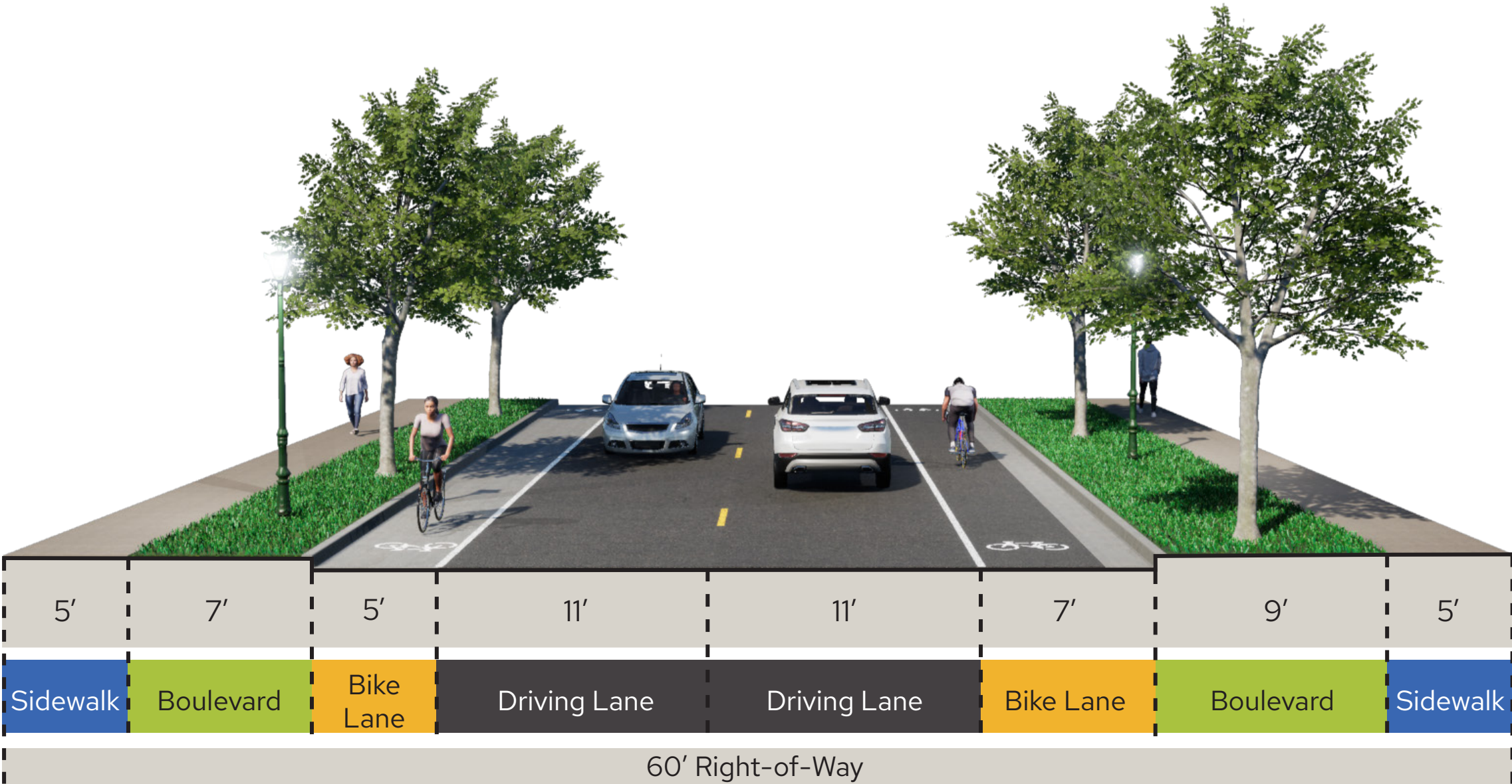
On-Street Bike Lanes
