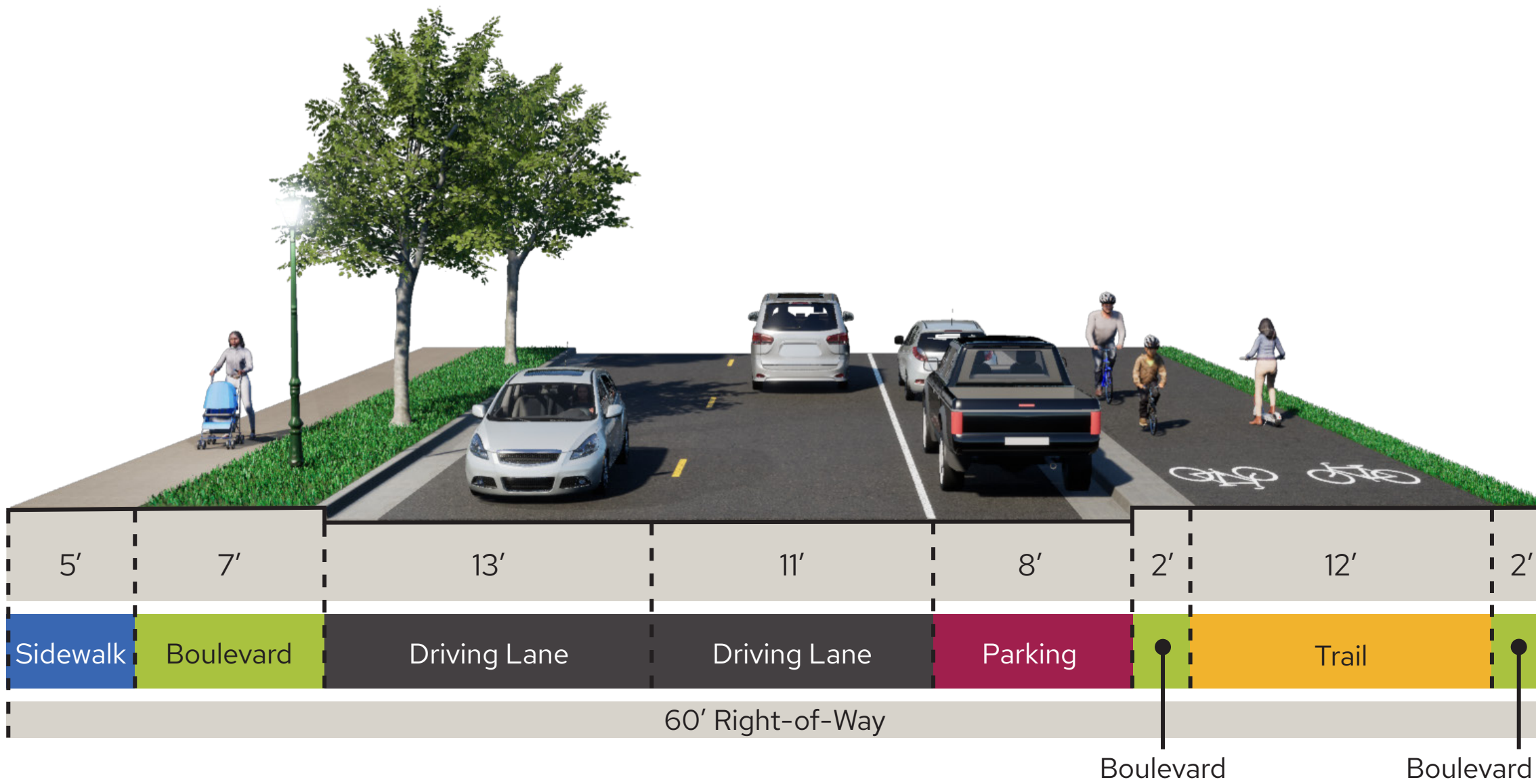
Off-Street Trail with a Parking Bay
