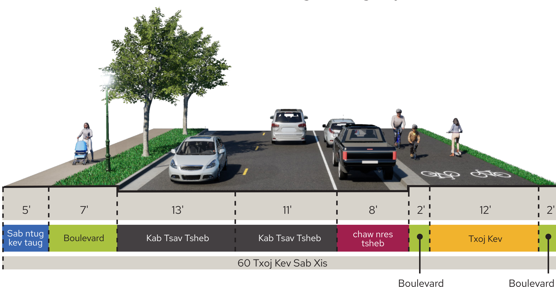
Off-Street Trail nrog Parking Bay
