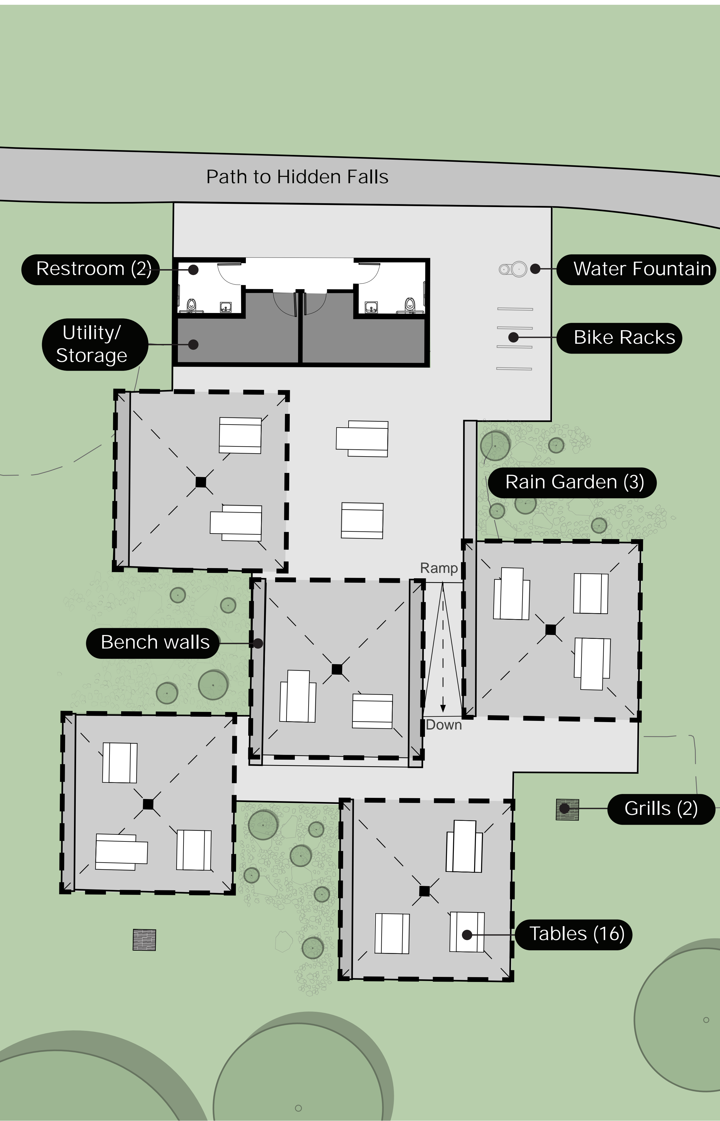
Pavilion Plan
