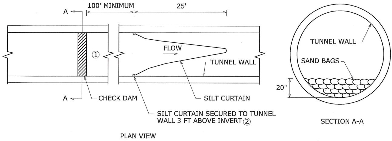
CHECK DAM/FLOATATION SILT CURTAIN
