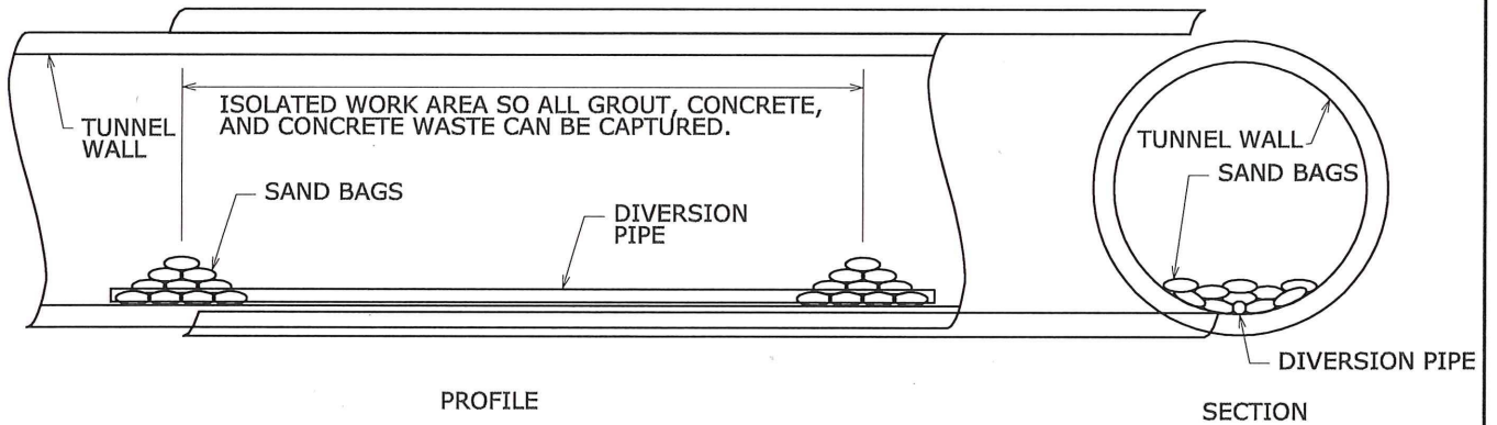
CHECK DAM
