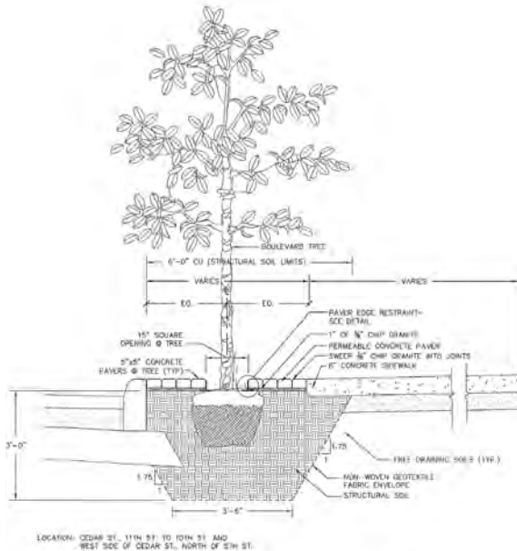
1 BOULEVARD TREE PLANTING W/ PERMEABLE PAVERS - SECTION
